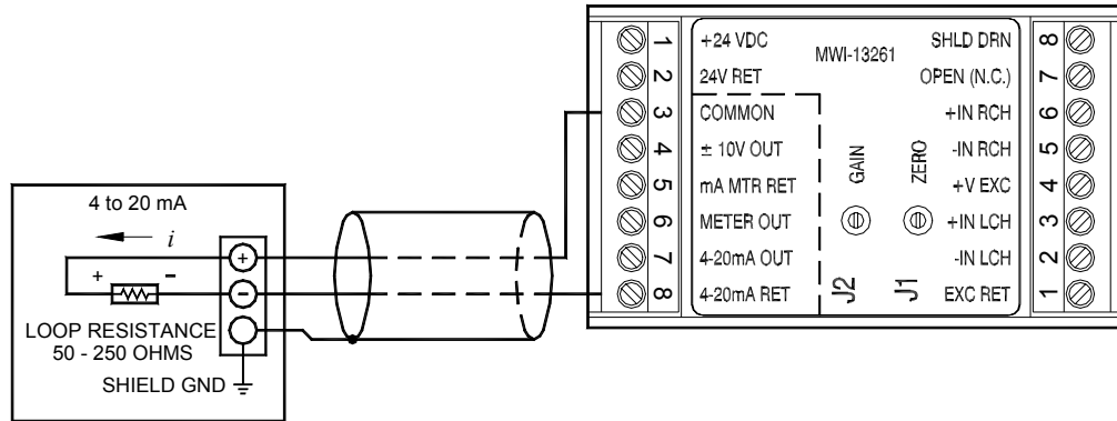
Figure 10 – 4-20 mA Output Wiring for Ground Referred Burden
