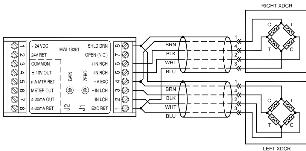
Figure 5 - Full-bridge Transducer Wiring
