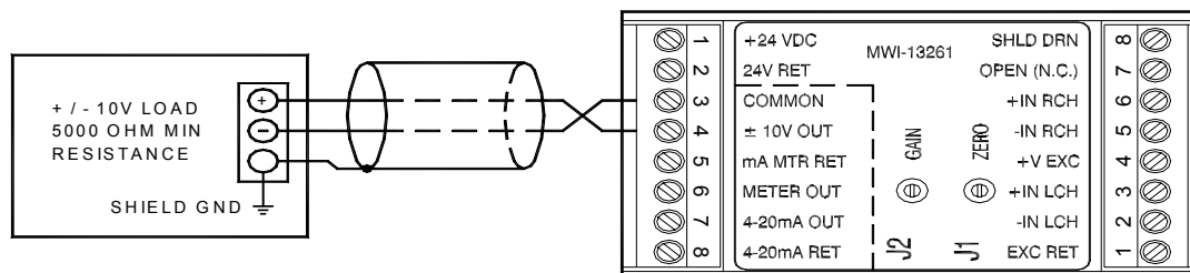
Figure 7 - Output Wiring, +/- 10V Analog
