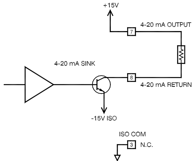
Figure 9 – 4-20 mA Output Circuit Wired for Floating Burden
